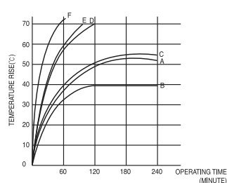
〈Fig. 8) INTERMITTENT OPERATION OF S9R40GD(WITHOUT GEAR HEAD)
