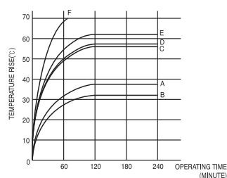
〈Fig. 6) INTERMITTENT OPERATION OF S7R15GD(WITHOUT GEAR HEAD)
